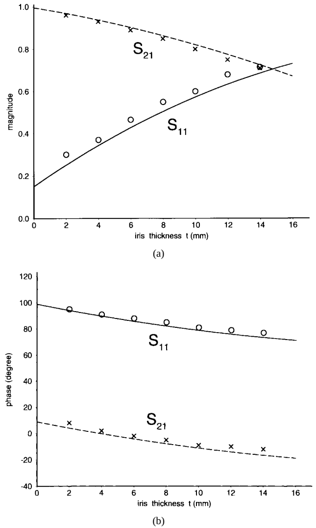
Fig. 3. Plots of: (a) magnitudes and (b) phases of scattering coefficients against iris thickness predicted by present LSBRM model (— for s_{11} and --- for s_{21} ) and CCPT model of Shen and MacPhie [6] (o o o for s_{11} and x x x for s_{21} ) for thick eccentric iris with a = 12.7 mm, b = 9.5 mm, d = 1.5 mm, \theta = 0^\circ , f = 9 GHz.
